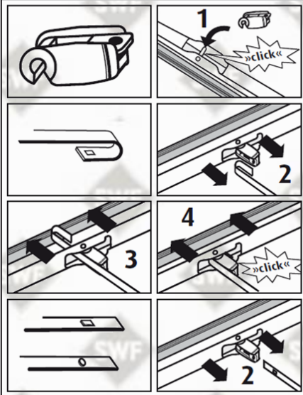
Montage / Fitting R
