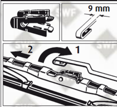
Montage / Fitting T2
