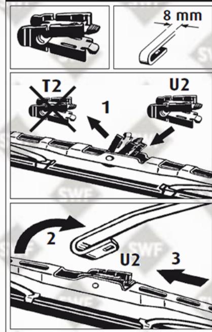
Montage / Fitting U2
