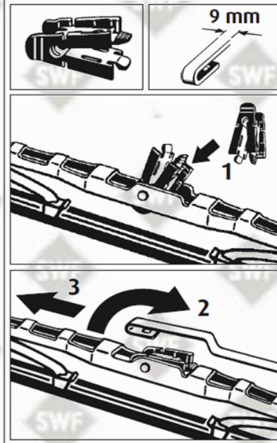
Montage / Fitting T2
